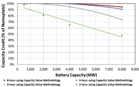
As shown, the longest duration discharge (red) retains more than 90% of its capacity value than the shortest (green)
